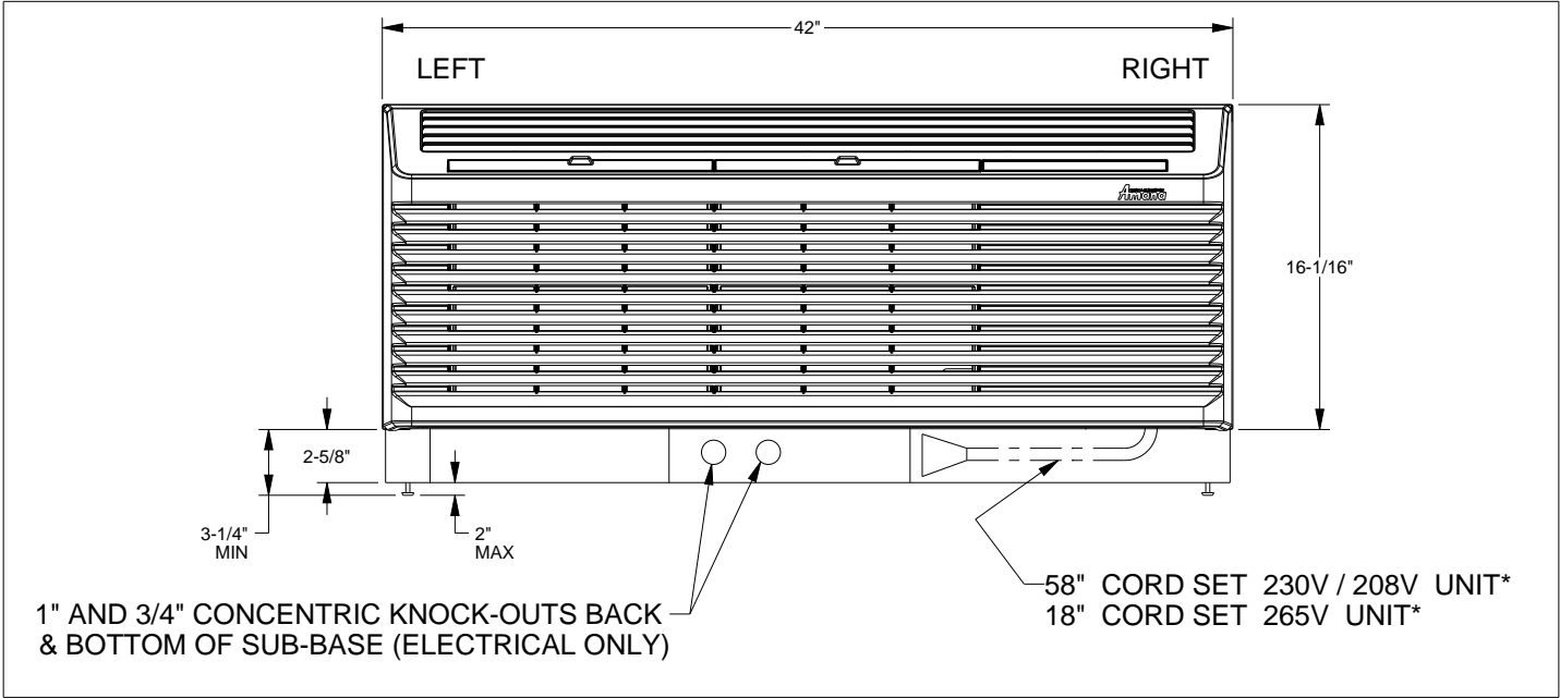
FRONT VIEW
