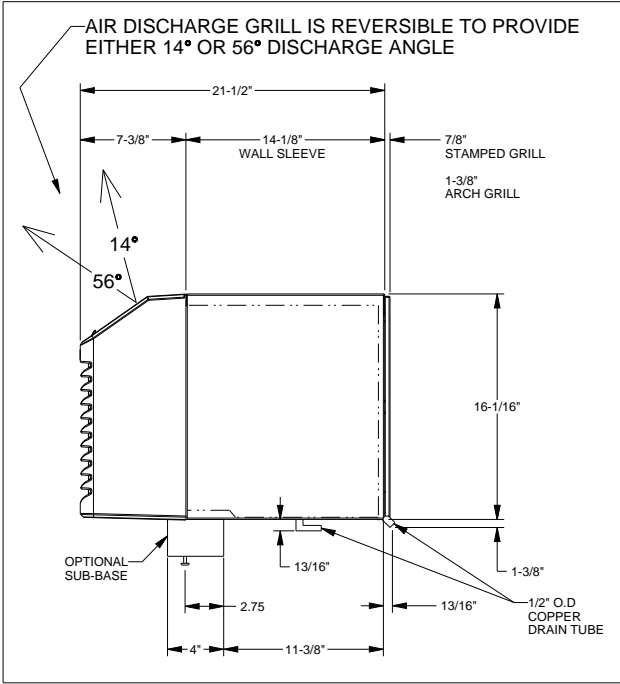
RIGHT VIEW
